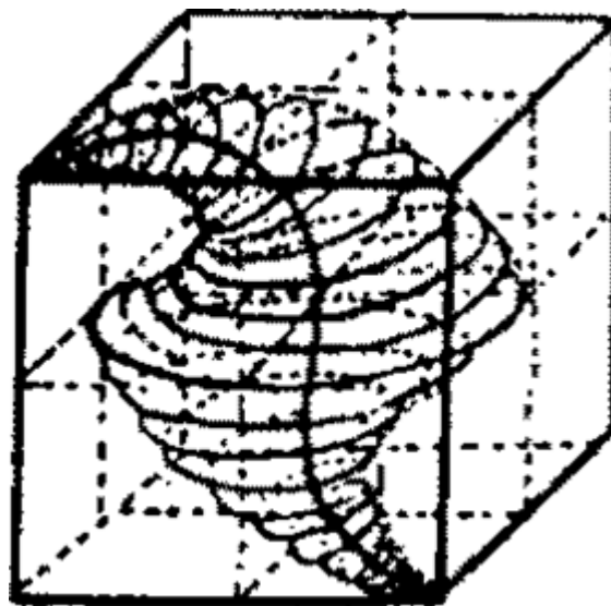
Fig. 49 Wave spirals on their wave shaft
