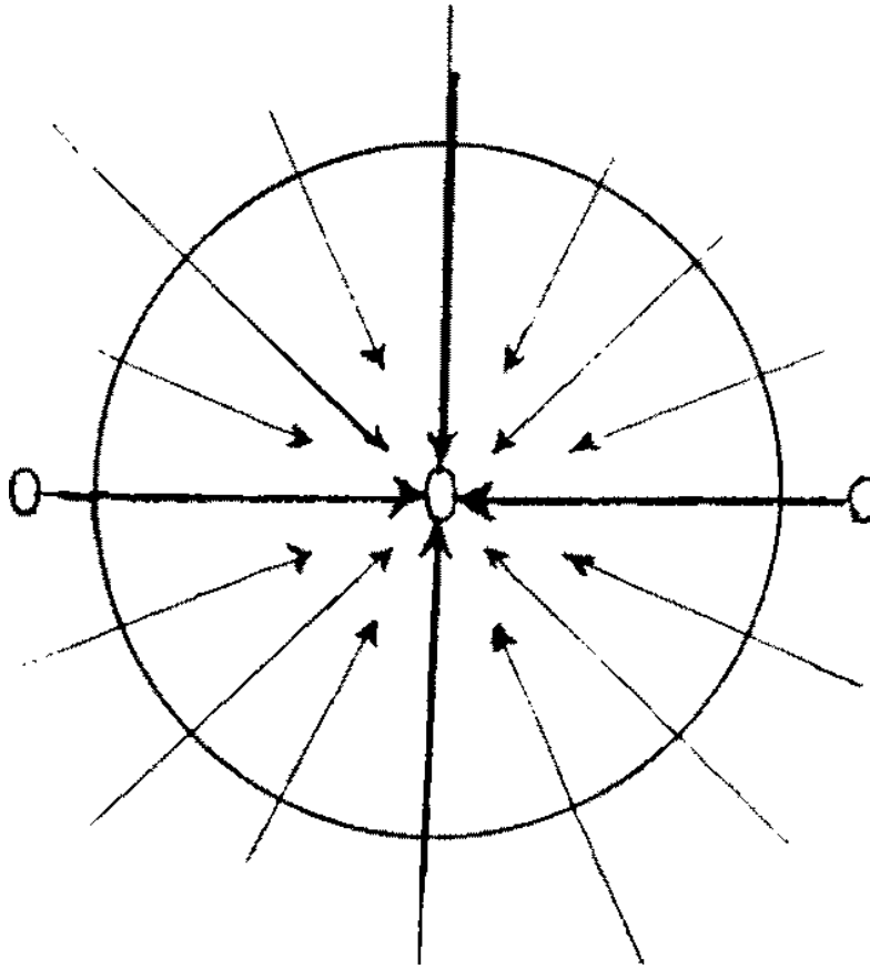
Fig. 59 Illustrating the radial universe concept.
