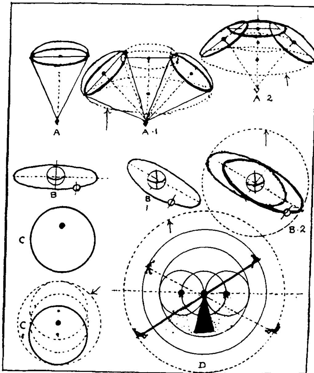
FIG. 46. Every thought and action in this universe is centered by its energy Source, which controls its actions and thoughts from within and balances them from without by two extensions of that center . These extended poles are the ends of gravity shafts around which all masses rotate under true circular control. A—represents a spinning top. B—the earth's orbit. C—a wheel with a shaft off-center. D—a seesaw. See text.
