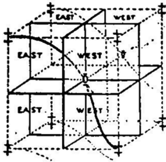
Fig. 48 The six inner mirrors of radiation.
