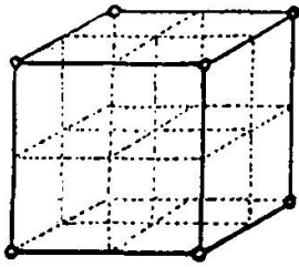
Fig. 5 Mirror planes of reaction
