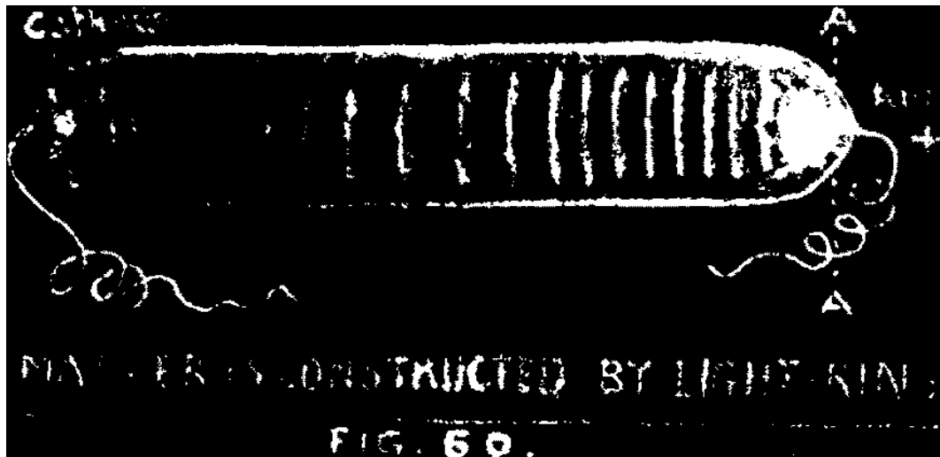
Electricity records Mind-thought in rings of light which spin around a Magnetic center of still, invisible light. All motion in all the universe spins around Mind-centers which becomes shafts as motion extends
