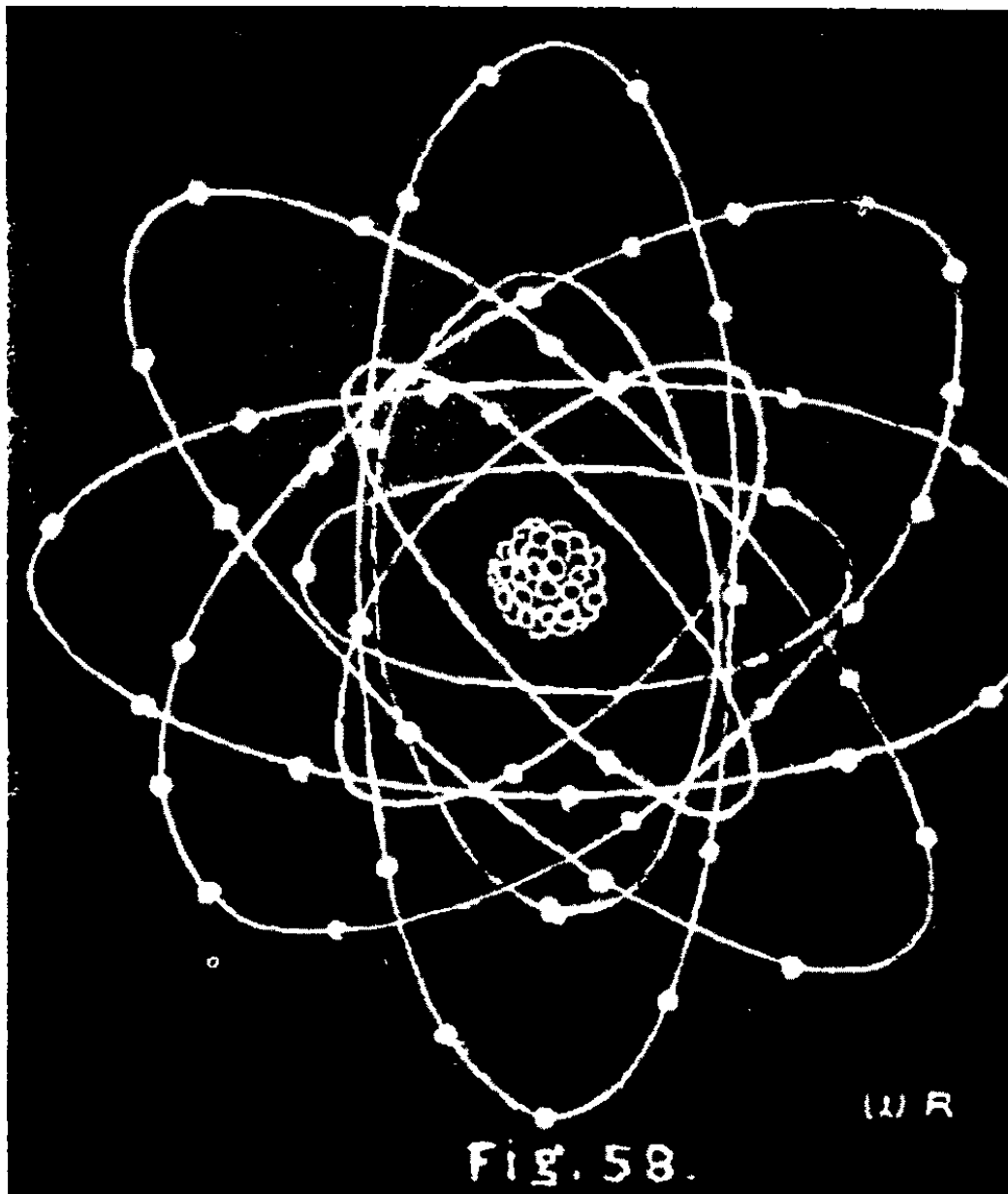
The Rutherford Bohr atom.
