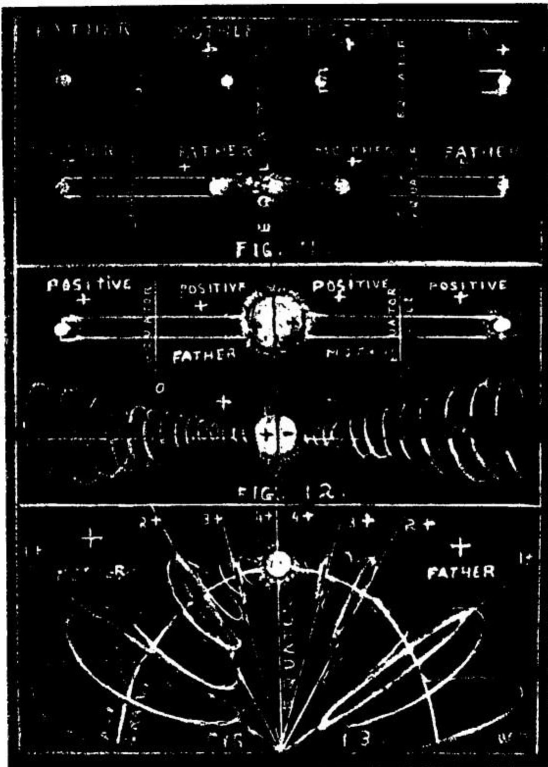
Illustrating the Father-Mother Principle of building bodies by dividing light into polarized units, and reproducing bodies by uniting two oppositely projected units into one by centripetal compression. POLARITY and sex are ONE . Sex and electric potential are ONE .
