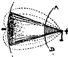
Fig. 25 A & B Interchange between un- equal volumes
