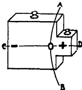
Fig. 22 Interchange between un- equal opposites
