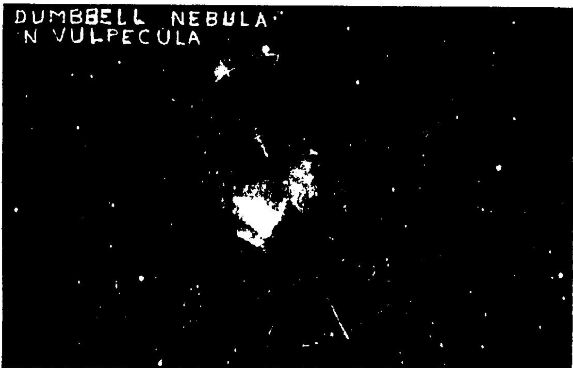
Fig 148 Illustrating the death principle in all matter. Spheres are created by compressing rings to form in them. Spheres are then disintegrated by projecting rings from them until a black hole surrounds their axis of rotation and they gradually expand until they eventually disappear into their cathodes.
