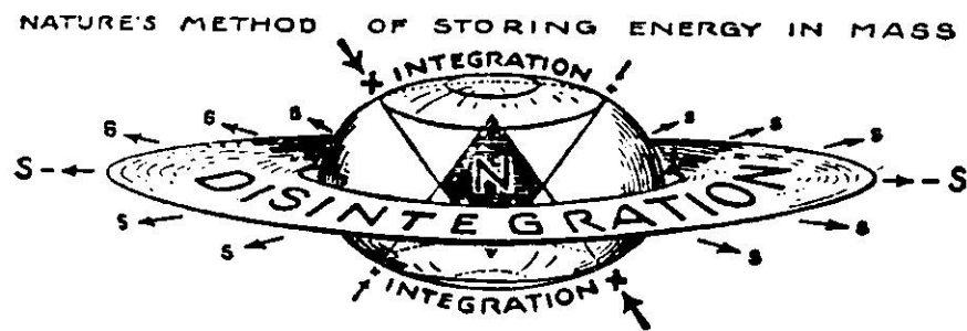
Fig. 65 As poles flatten equators lengthen
