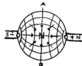
Fig. 27 Matter is formed between opposite poles in waves
