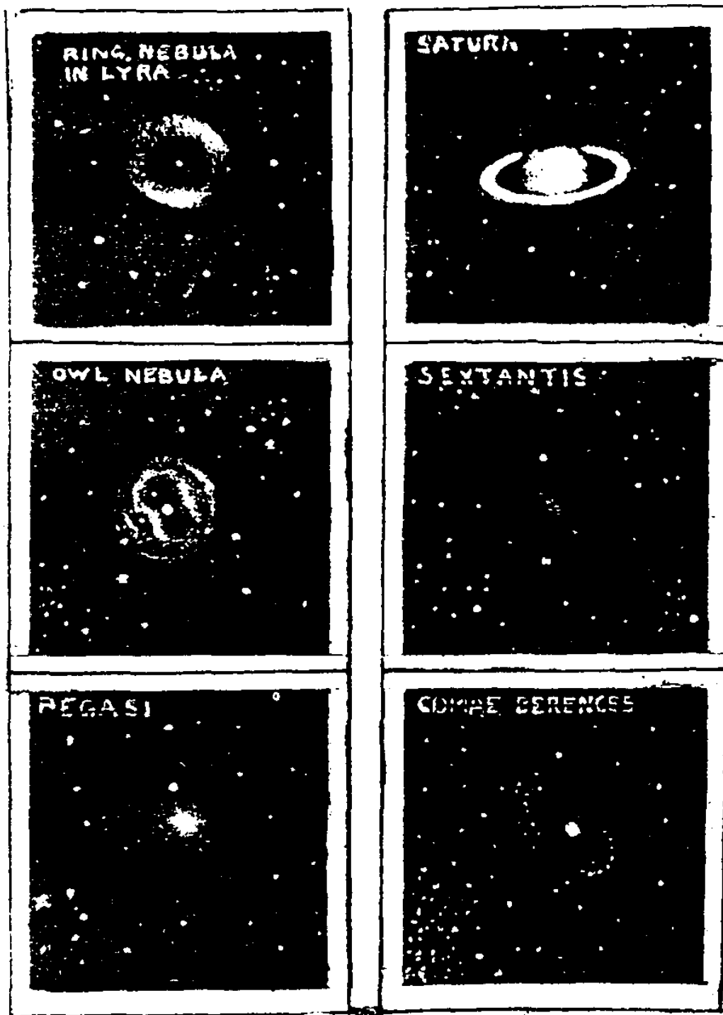
FIG. 32 The centering shaft, around which suns rotate, again compresses another sun into its vortex to repeat the process until all its mass disappears as rings. Lyra and Hydrae nebulae are good examples in the stellar system and Saturn well exemplifies how planets in our solar system, disappear into their zero.
