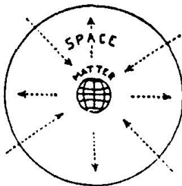
Fig. 22 Interchange between un- equal opposites
